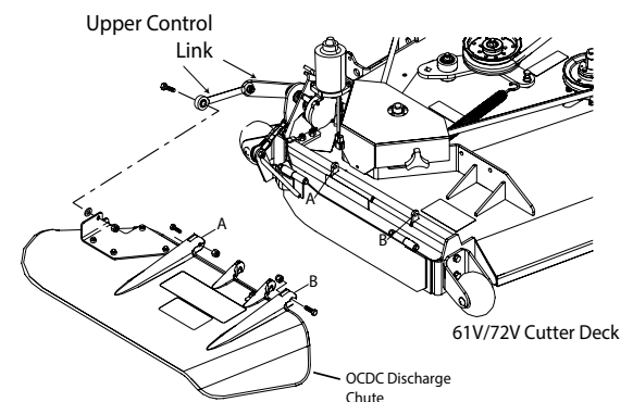
Figure 3-31. Discharge Chute Installation
