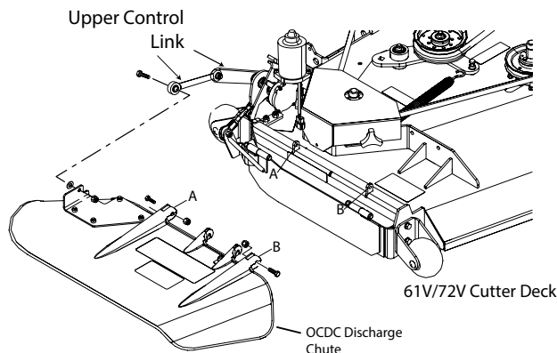
Figure 3-41. Discharge Chute Installation
