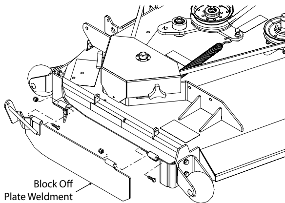
Figure 3-13. Block Off Plate Weldment Installation
