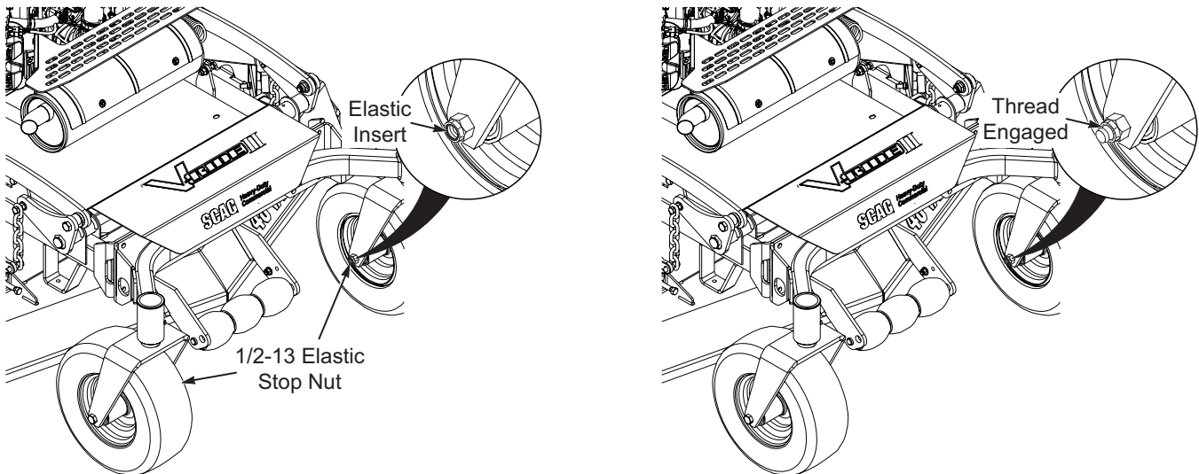
Figure 1. Front Axle Caster Bolt & Elastic Locking Nut
