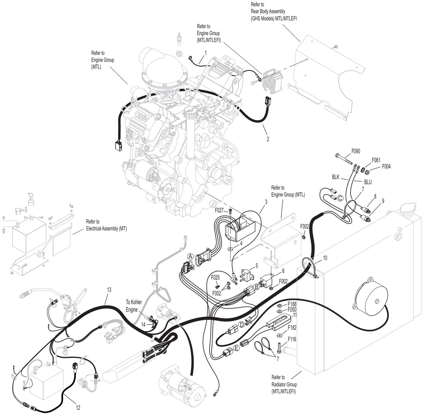
DETAIL A
